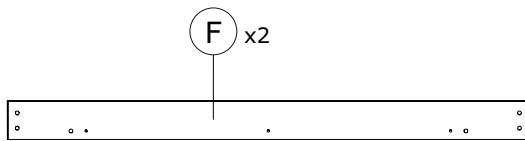
FS3868 901x62x38mm
